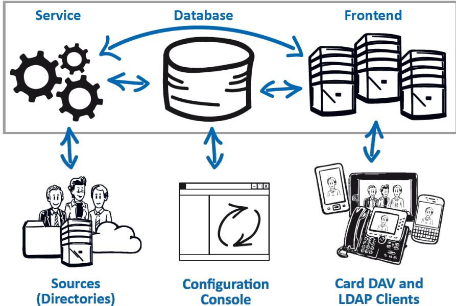
Figure 1: PeopleSync Architecture
