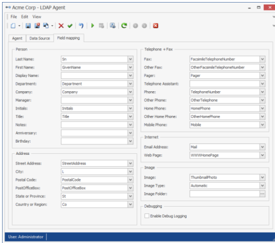
Figure 25: LDAP Agent field mapping
