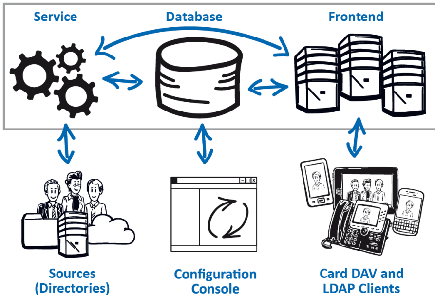
Figure 1: PeopleSync Architecture
