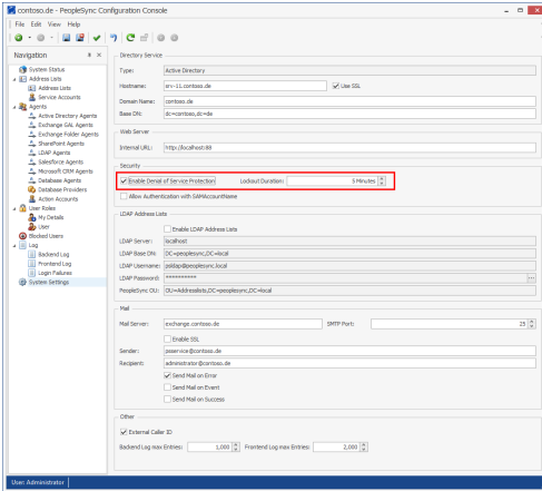
Figure 12: Configuring DoS protection
