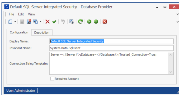
Figure 32: Custom Database Provider
