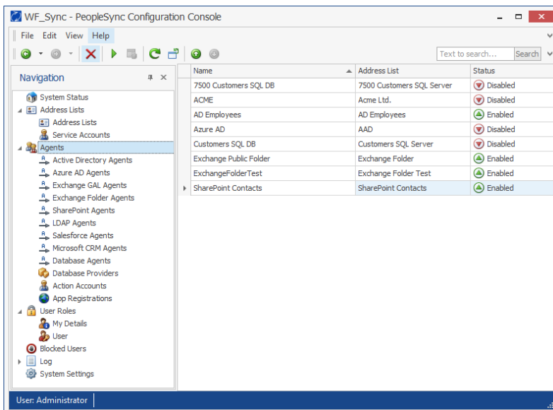
Figure 17: List of Agents
