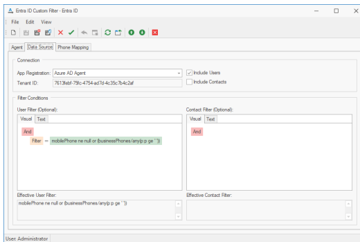
Figure 25: Entra ID Agent Configuration
