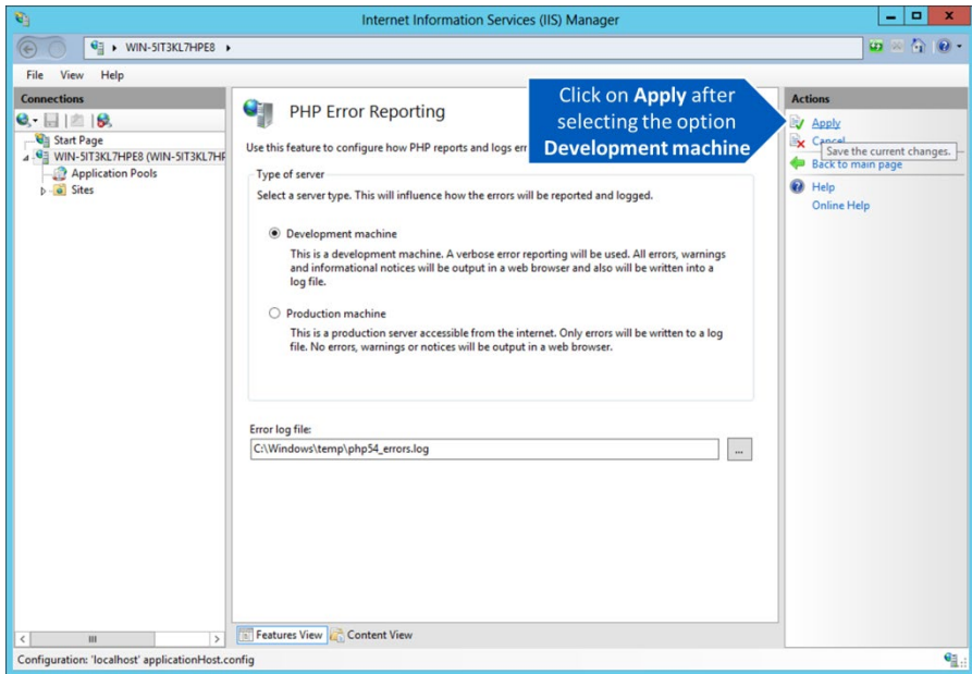
Figure 38: IIS Manager PHP Error Reporting
