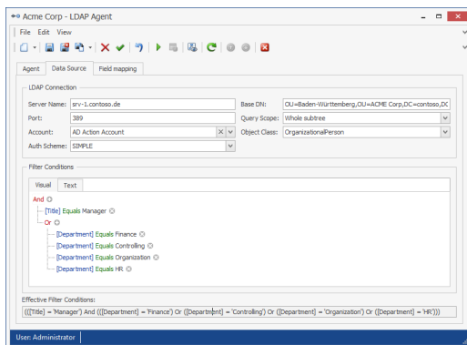
Figure 30: LDAP Agent Configuration
