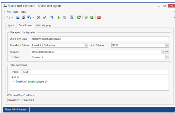
Figure 28: SharePoint Agent Configuration
