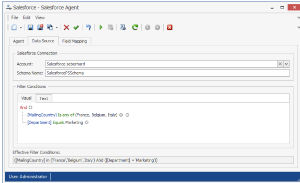
Figure 34: Salesforce Agent Configuration
