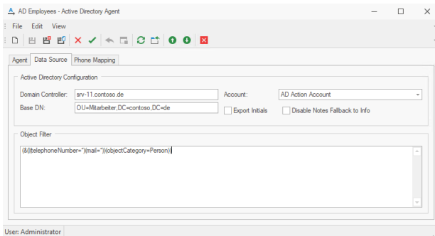
Figure 24: Active Directory Agent Configuration
