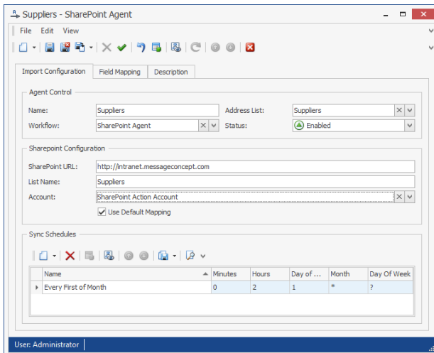
Figure 25: SharePoint Agent Configuration
