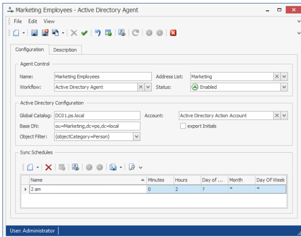
Figure 22: Active Directory Agent Configuration
