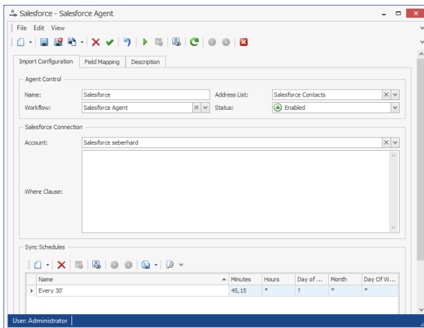
Figure 29: Salesforce Agent Configuration
