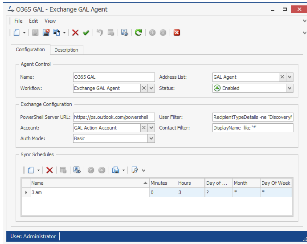
Figure 23: Exchange GAL Agent Configuration
