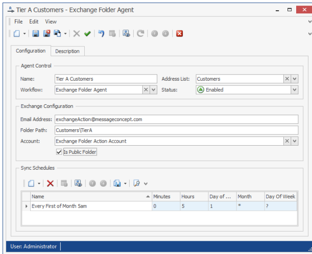
Figure 24: Exchange Folder Agent Configuration
