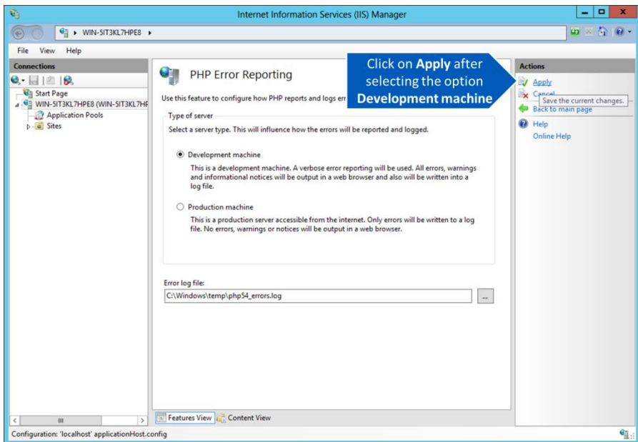
Figure 33: IIS Manager PHP Error Reporting
